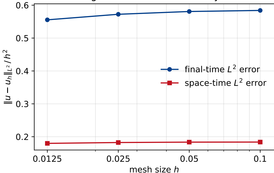
Burgers: L^2 error rescaled by h^2
