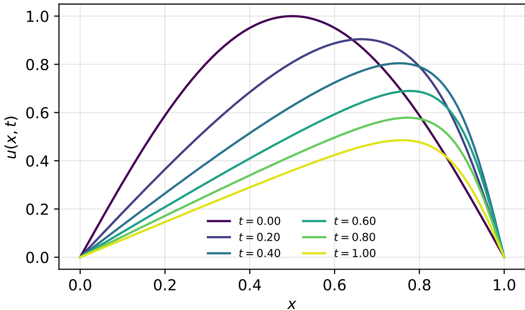
Forward Burgers: nonlinear steepening ( \nu = 0.05 )
