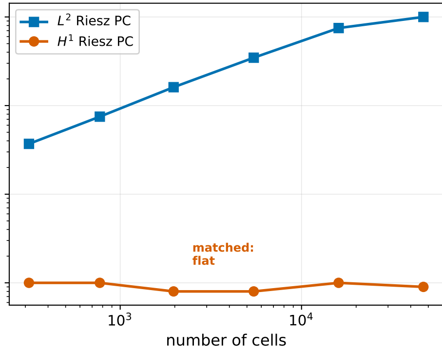
H^1 -regularised problem
