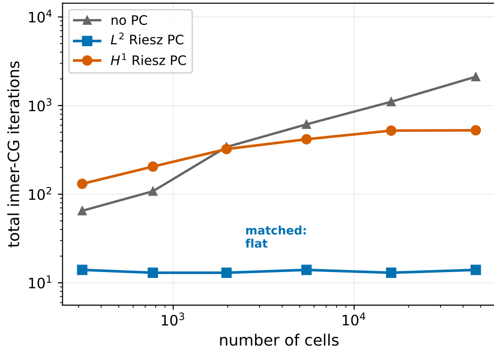
L^2 -regularised problem
