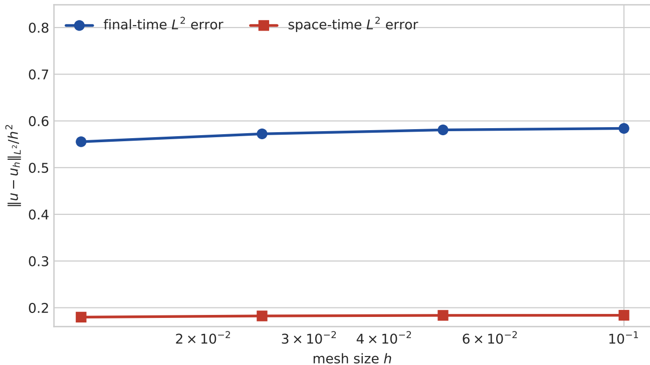
Burgers: L^2 Error Rescaled by h^2
