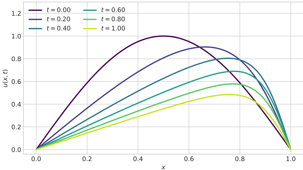
Forward Burgers: Nonlinear Steepening ( \nu = 0.05 )
