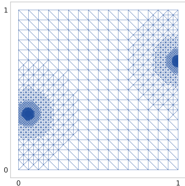
Mesh Graded Towards Both Features 3775 Cells, h_{\max}/h_{\min} = 32 , L^2 Error 7.3\text{e-}04
