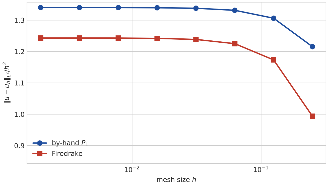
Poisson: L^2 Error Rescaled by h^2
