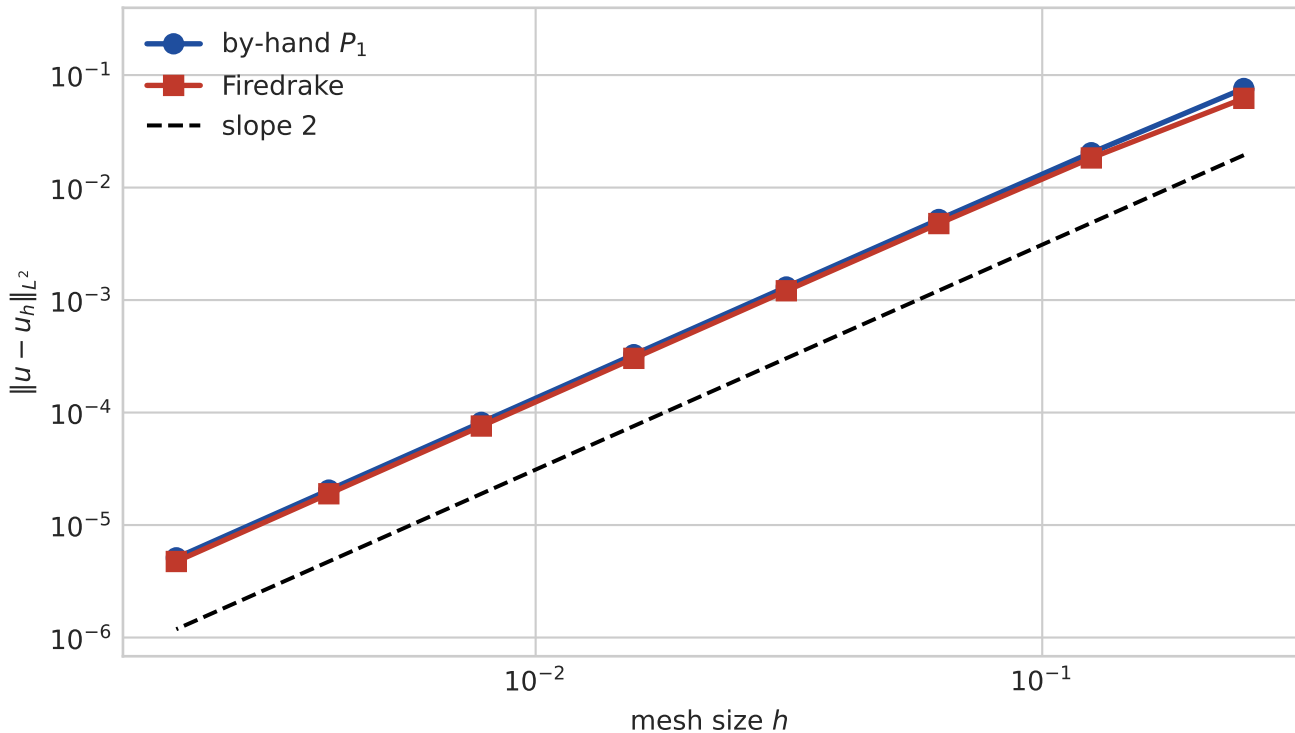
Poisson: Manufactured-Solution Convergence
