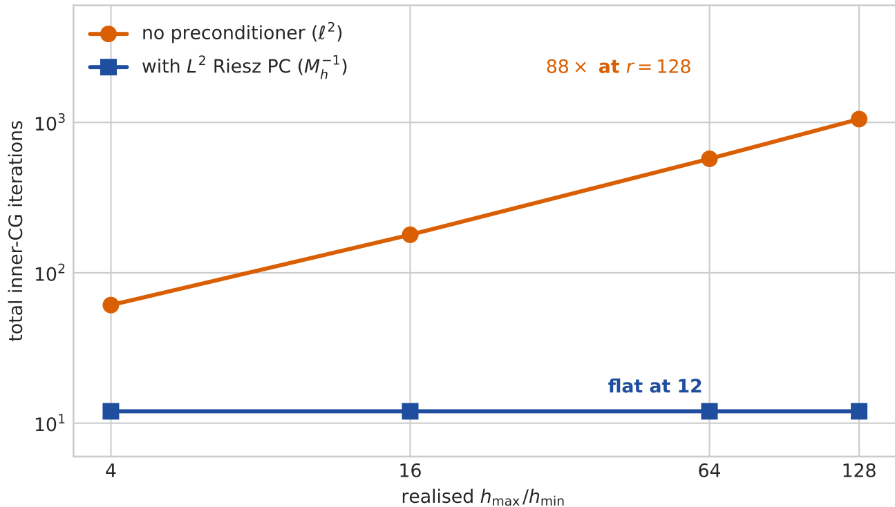
Inner-CG Iteration Count With and Without the Riesz Map
