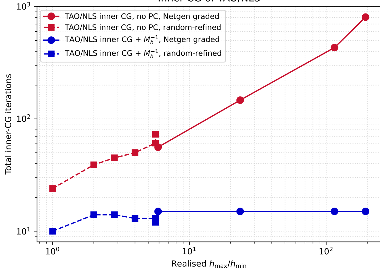
Inner CG of TAO/NLS
