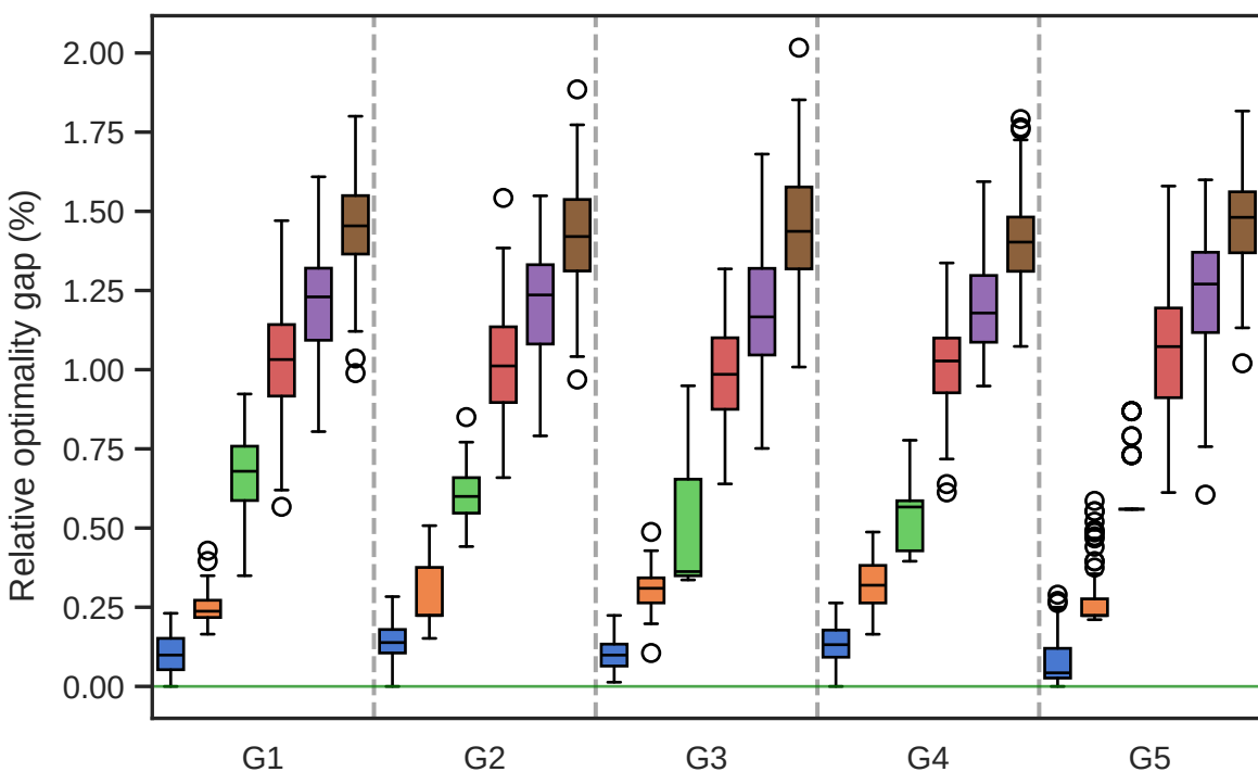
(b) Max-4-Cut
