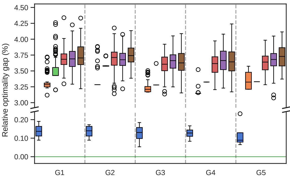
(b) Max-4-Cut
