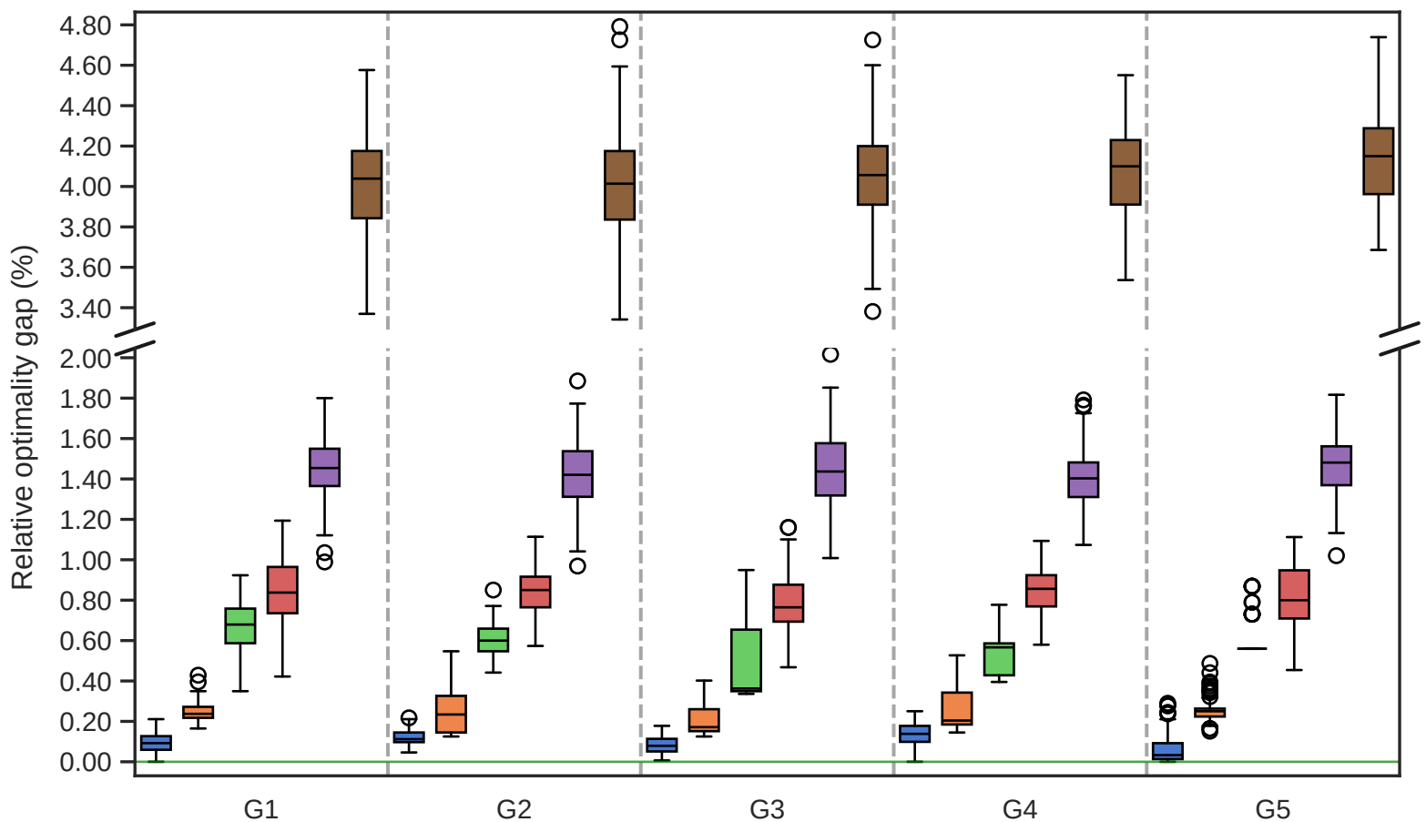
(b) Max-4-Cut
