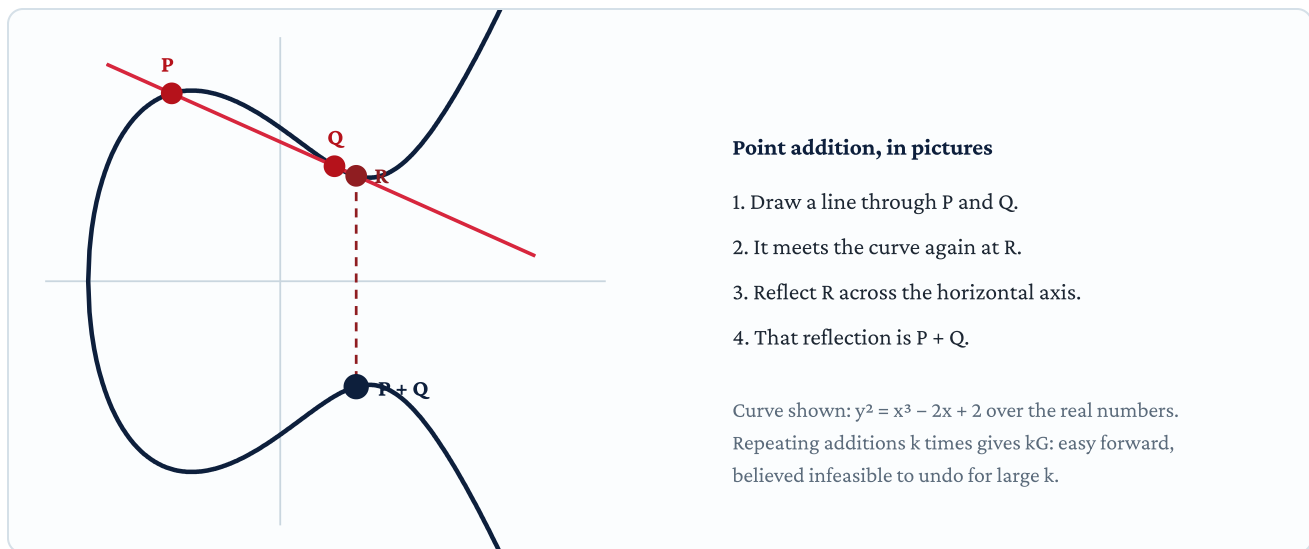
Figure 2.1 The geometric idea behind elliptic curve point addition. Real cryptographic curves use the same rules over a finite field.
