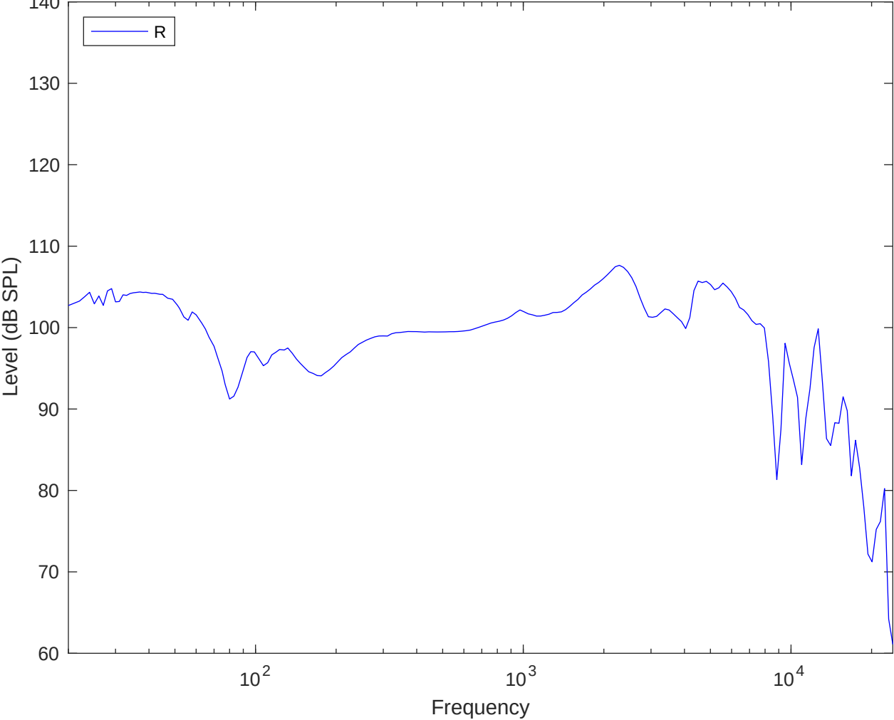
Transfer Function for mcdermott-BLACK-Soundcard-6-25-2024
