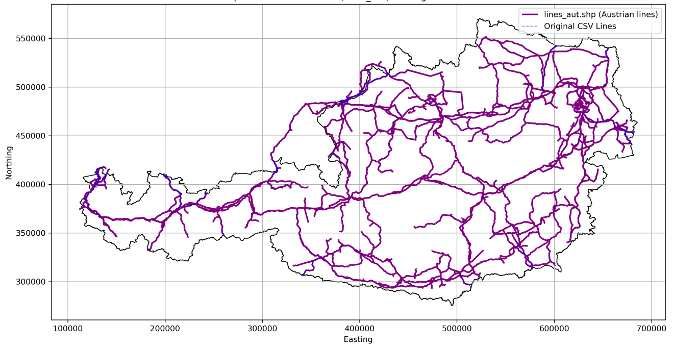
Comparison: Austrian Grid (lines_aut) vs Original 380kV Lines
