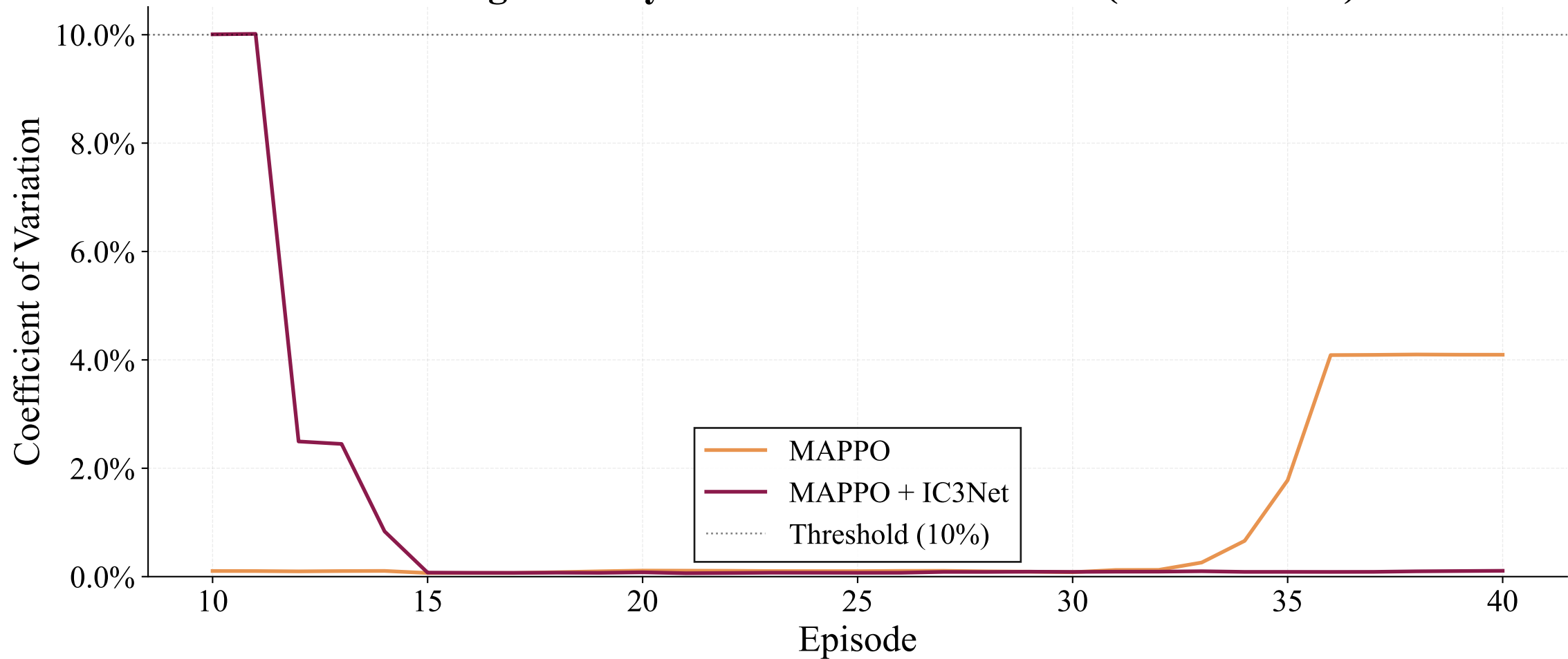
Training Stability: Coefficient of Variation (Eval Reward)
