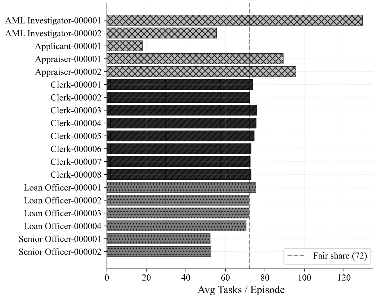
Shortest Queue
