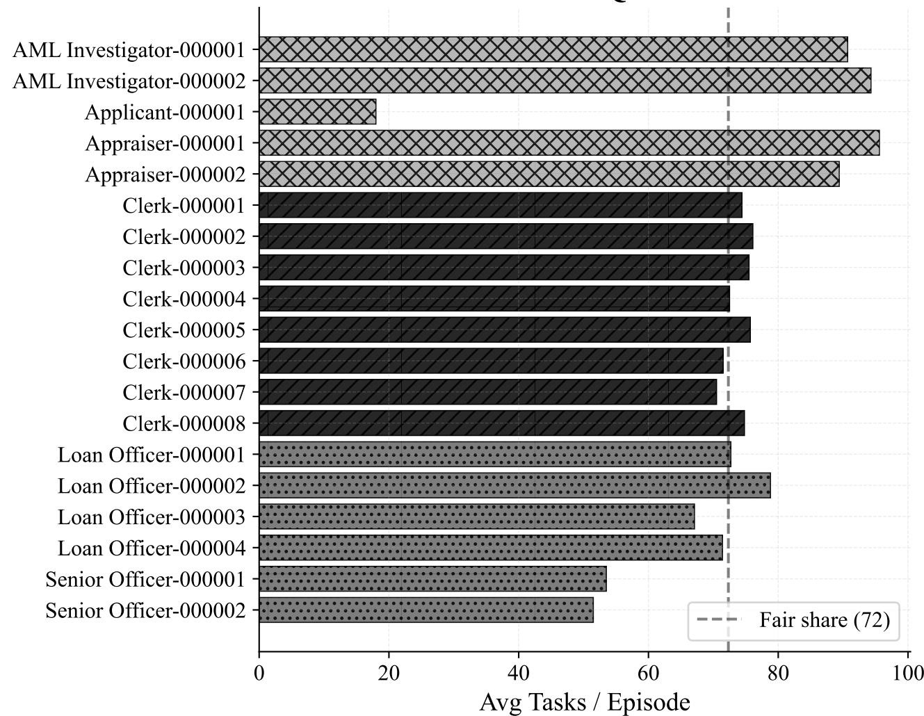
Shortest Queue
