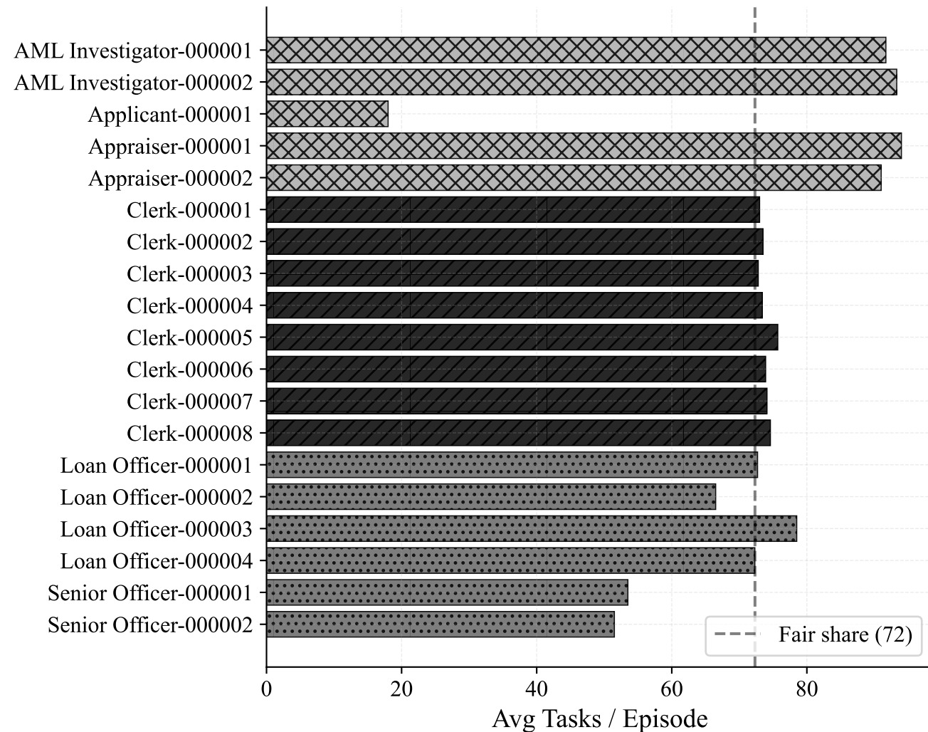
Best Median
