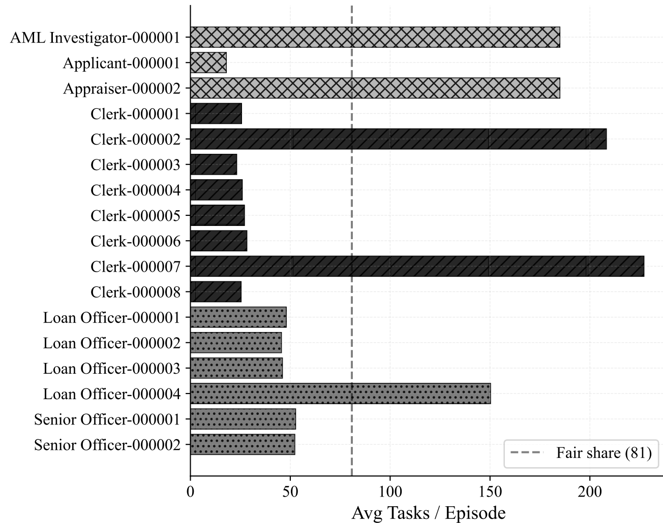
Best Median
