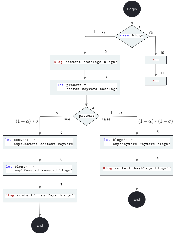
Fig. 8. Control flow graph generated from function body of running example 2.
