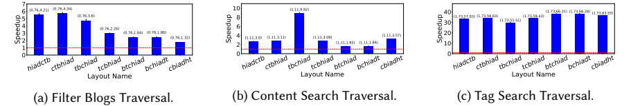
Fig. 10. Performance comparison of M_{Solver} with MLTON. The tuple on top of each bar shows the median runtime in seconds of M_{Solver} followed by the corresponding layout when compiled with MLTON.
