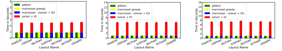
(a) Compile times for the Filter blogs traversal.
