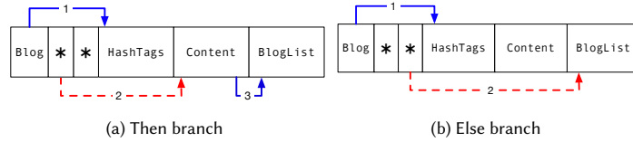
Fig. 5. Optimized layout with favorable access patterns.
