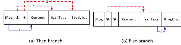
Fig. 4. Representation with pointers to allow random access.
