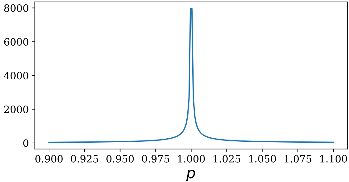
Condition number
