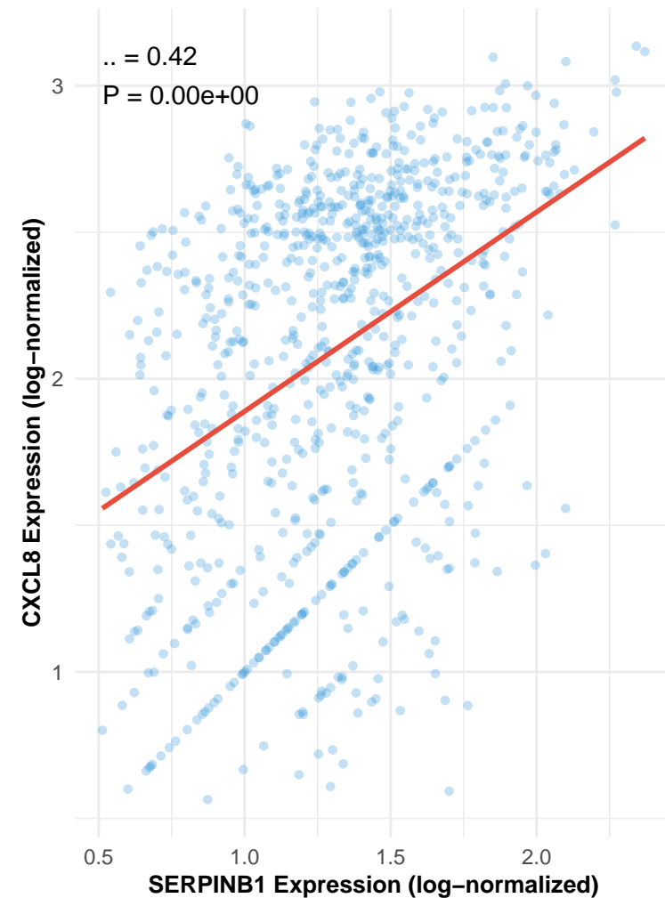
SERPINB1 vs CXCL8
