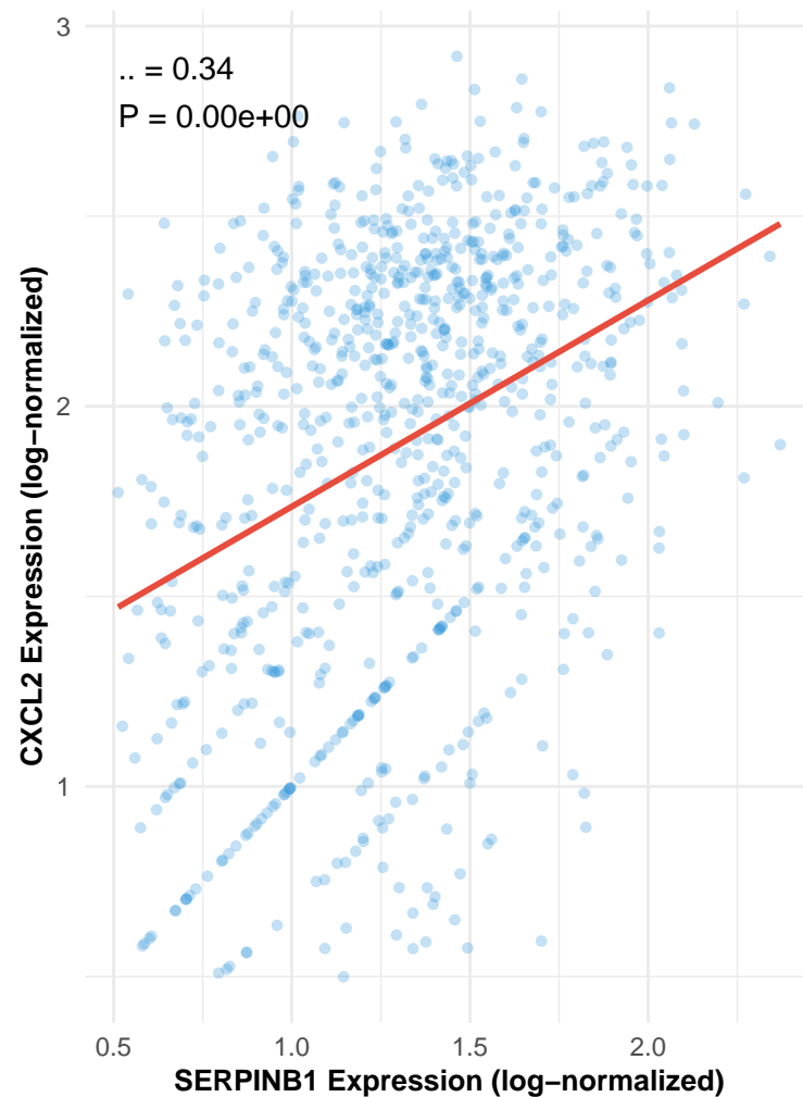
SERPINB1 vs CXCL2
