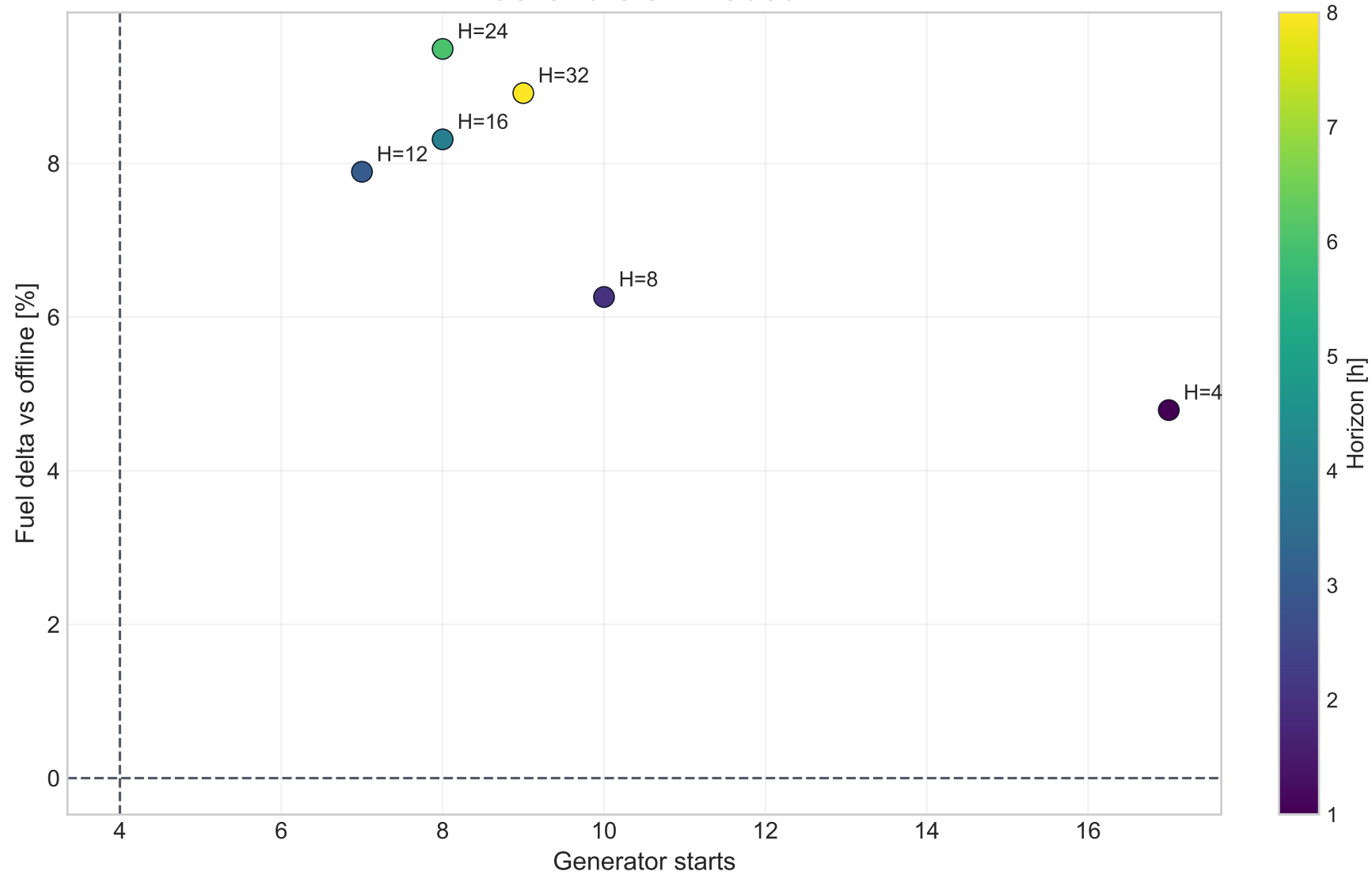
Fuel and Start Tradeoff
