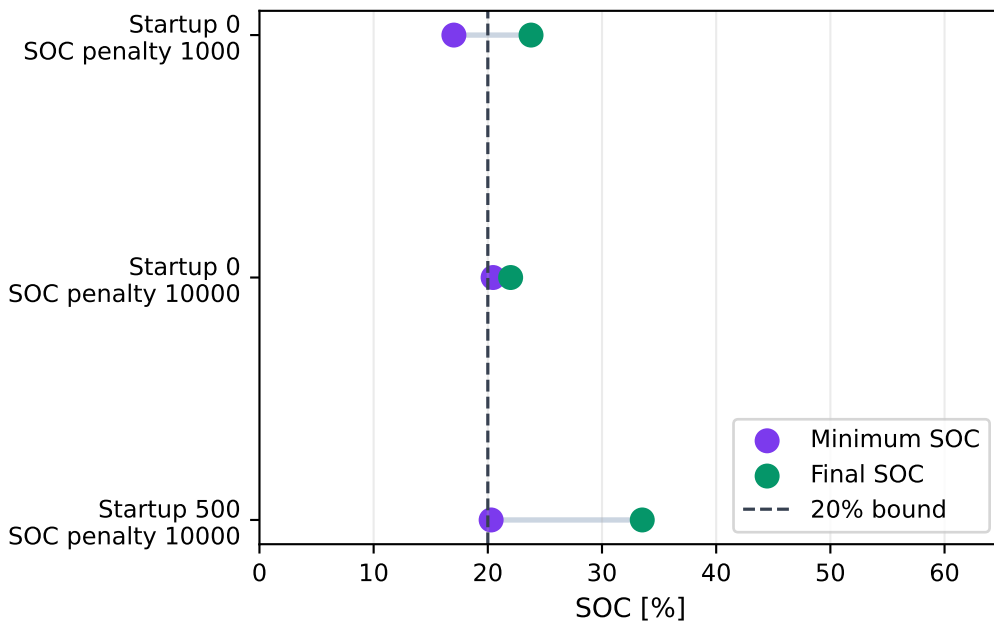
SOC Outcome
