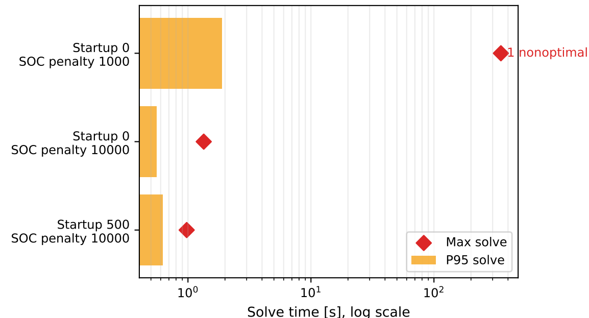
Solve Robustness
