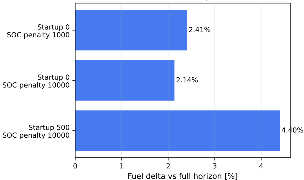
SOC Outcome
