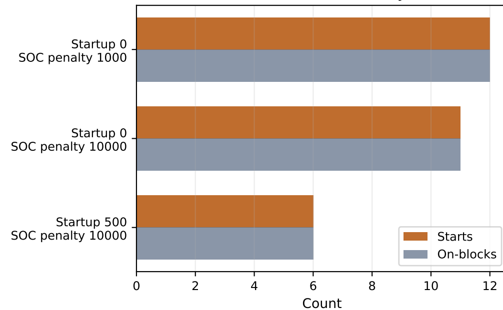
Solve Robustness
