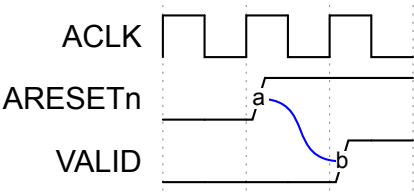
Figure A2.1: Exit from reset
