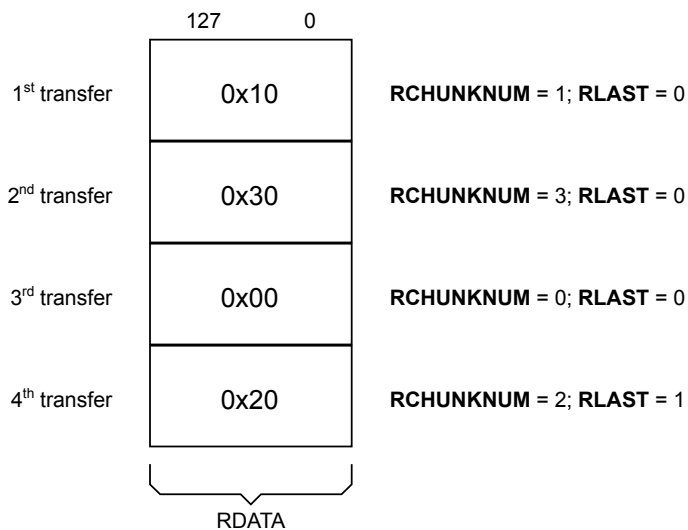
Figure A5.4: Example of a wrapping transaction
