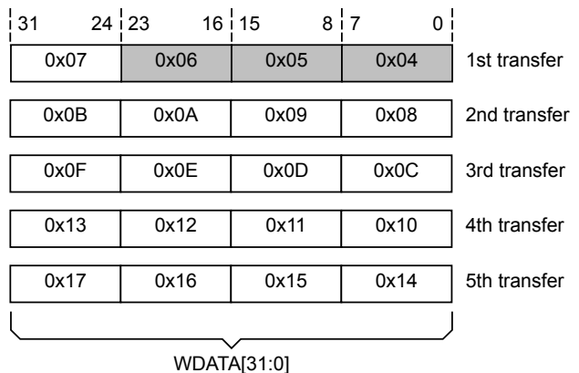
Figure A3.6: Aligned and unaligned transfers on a 32-bit data channel
