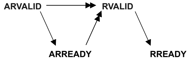
Figure A2.6: Read transaction handshake dependencies
