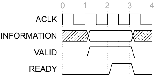
Figure A2.2: VALID before READY handshake
