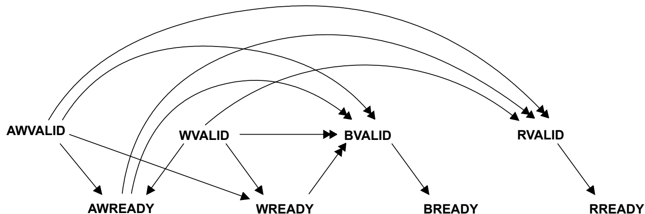
Figure A6.5: Atomic transaction handshake dependencies
