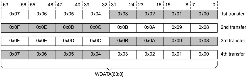
Figure A3.8: Aligned wrapping transfers on a 64-bit channel
