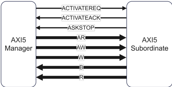
Figure A14.1: AXI5 interfaces using credit control signaling
