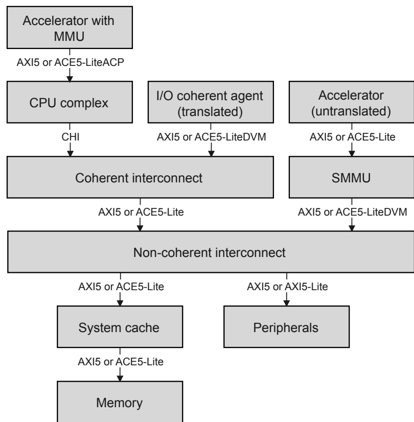
Figure B2.1: Example system topology showing possible interface classes
