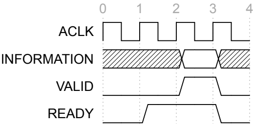
Figure A2.3: READY before VALID handshake
