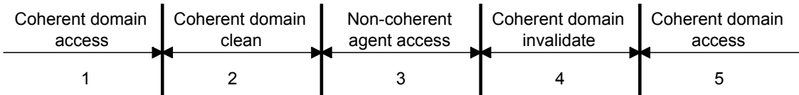
Figure A9.3: Required sequence of communication between coherent and non-coherent domains
