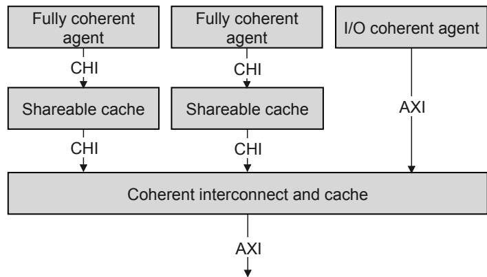
Figure A8.2: Example use of I/O coherency
