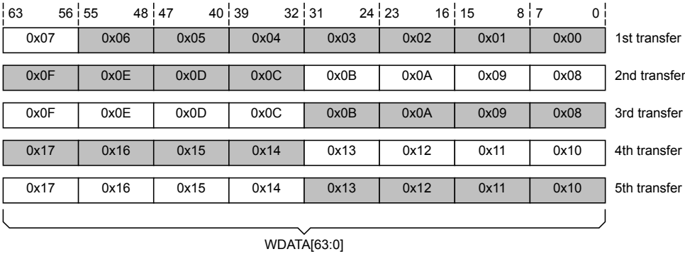
Figure A3.7: Aligned and unaligned transfers on a 64-bit data channel
