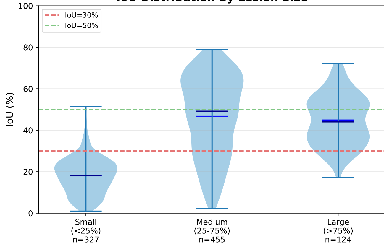
IoU Distribution by Lesion Size
