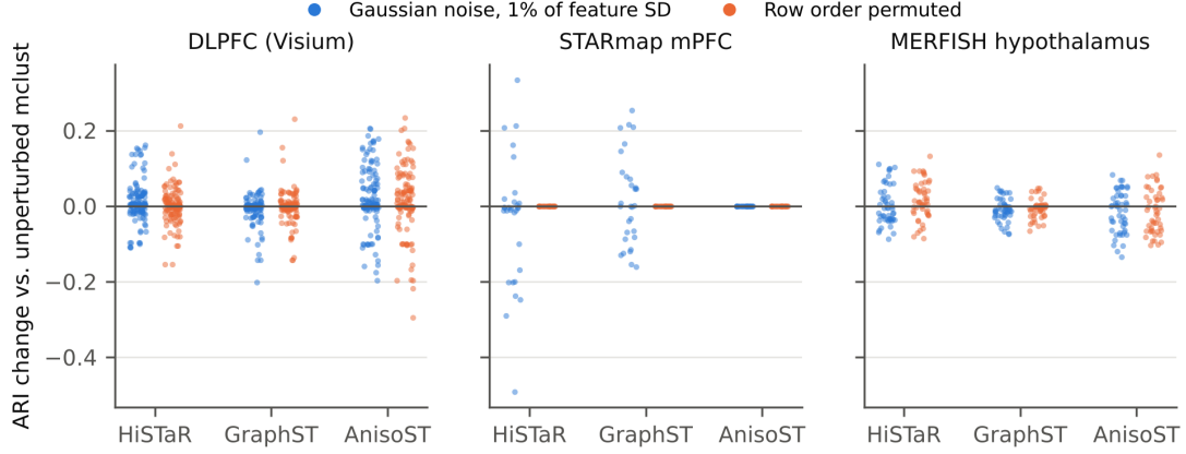
Fig. 2. Change in ARI of R mclust (EEE, default initialisation) when the same embedding is perturbed by permuting the spot order (orange) or adding noise at 1% of each feature’s standard deviation (blue); 10 perturbations per section and embedding.
