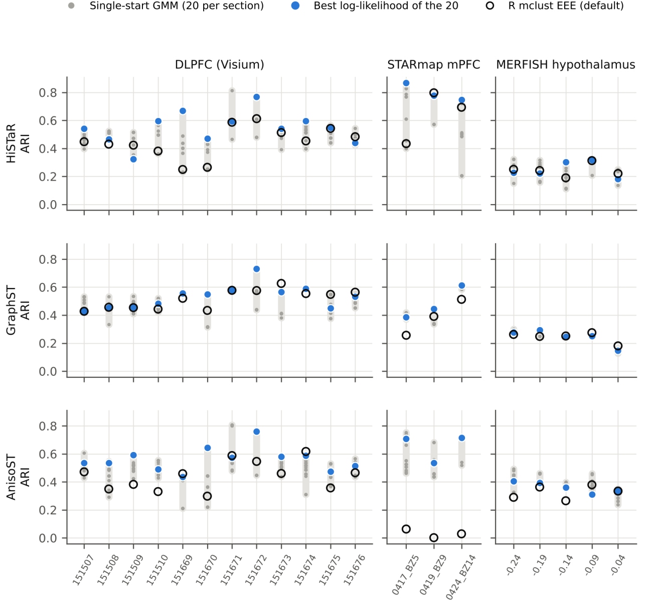
Fig. 1. The clustering lottery. For each section, one fixed embedding was clustered 20 times with a single-start tied-covariance GMM (grey dots; bar = range). Blue: the fit with the highest log-likelihood (label-free). Open circle: R mclust with default settings on the same embedding.
