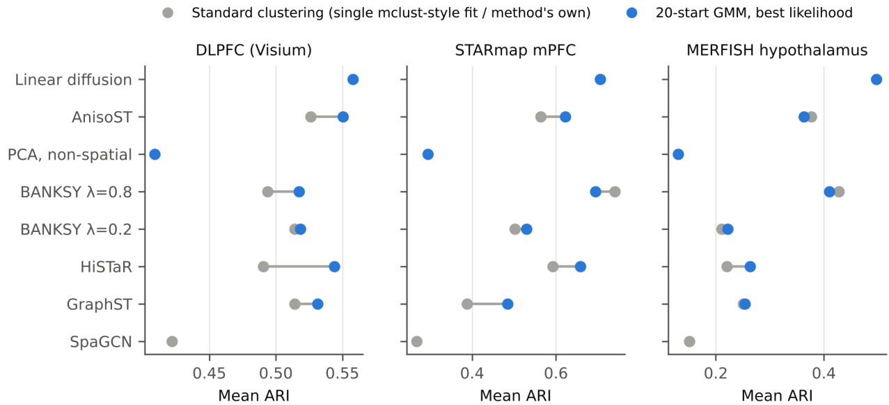
Fig. 4. Mean ARI per dataset with standard clustering (grey) and the 20-start, best-likelihood GMM (blue) applied to the same embeddings.
