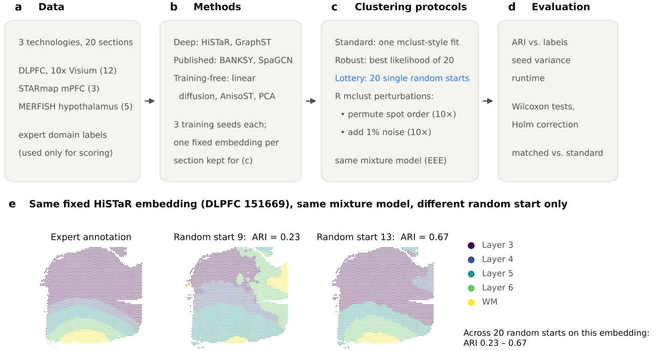
Fig. 1. Study design. a–d: data, methods, clustering protocols and evaluation. e: a real example of the clustering lottery. One fixed HiSTaR embedding of DLPFC section 151669 was clustered with the same tied-covariance Gaussian mixture from two different random starts; only the initialisation differs, yet ARI is 0.23 in one run and 0.67 in the other.
