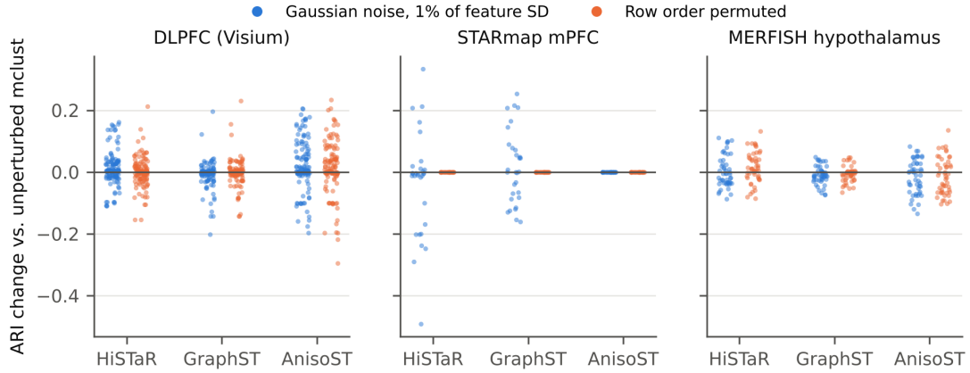
Fig. 3. Change in ARI of R mclust (EEE, default initialisation) when the same embedding is perturbed by permuting the spot order (orange) or adding noise at 1% of each feature's standard deviation (blue); 10 perturbations per section and embedding.
