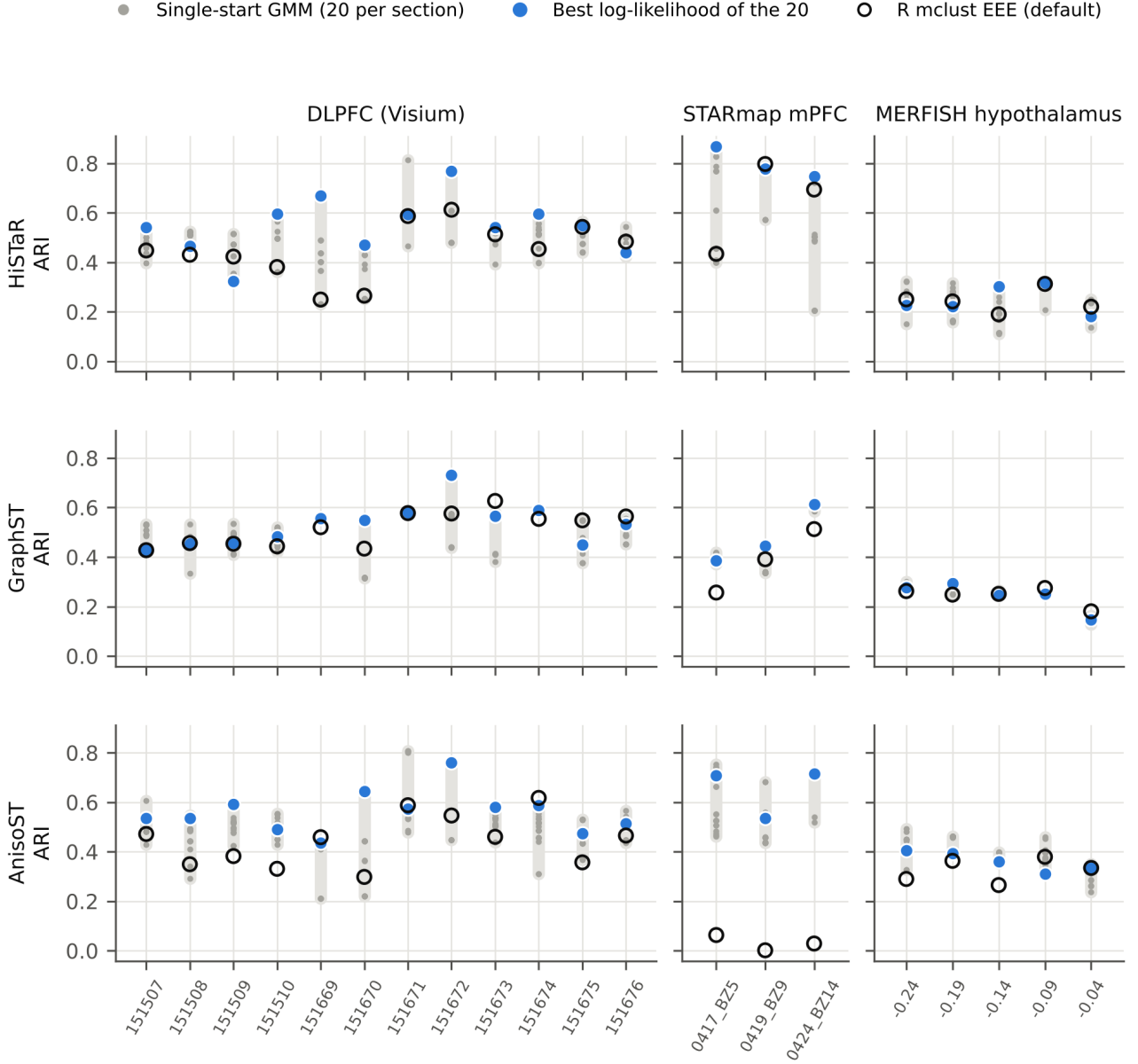
Fig. 2. The clustering lottery. For each section, one fixed embedding was clustered 20 times with a single-start tied-covariance GMM (grey dots; bar = range). Blue: the fit with the highest log-likelihood (label-free). Open circle: R mclust with default settings on the same embedding.
