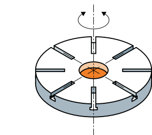
Swivel combination 90°/90°
