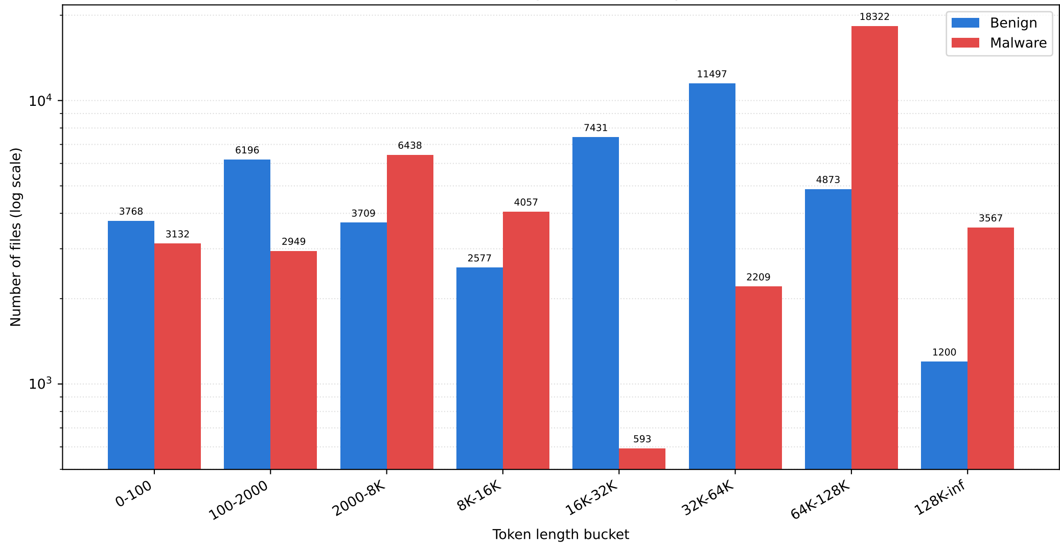
ELF file token-length distribution by class
