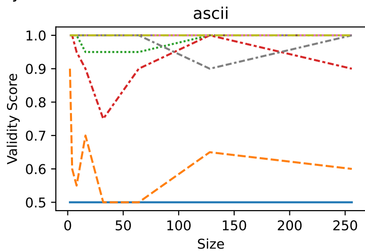
All Validity Score
