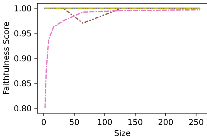
Int-n1000:1000
