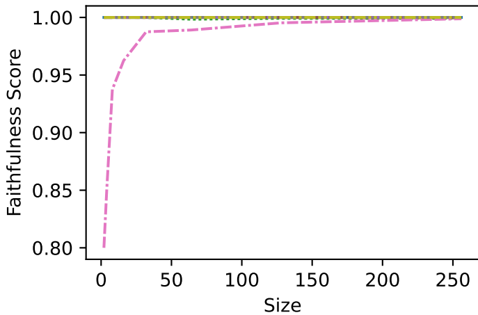
Int-10000000:10001000
