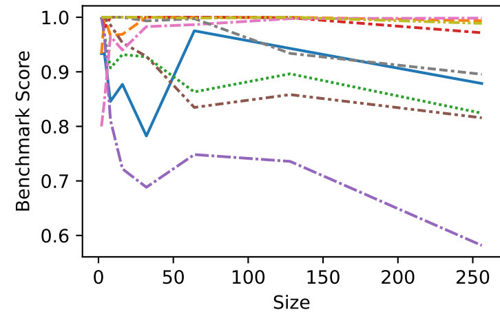
Int-10000000:10001000
