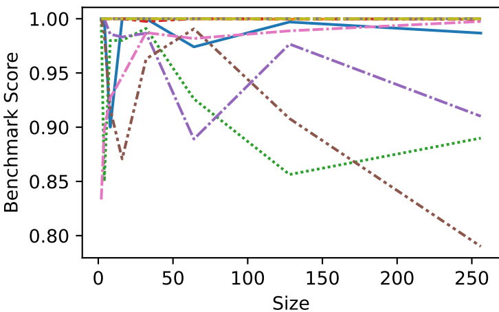
Int-n1000:1000
