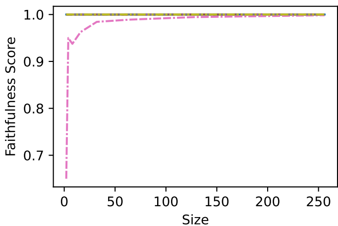
Float-10000000:10001000
