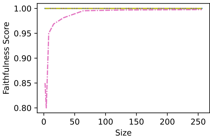
Int-10000000:10001000
