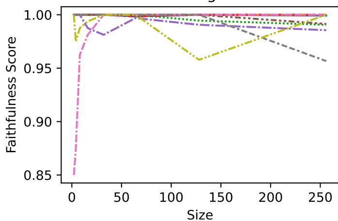
NumberWords
