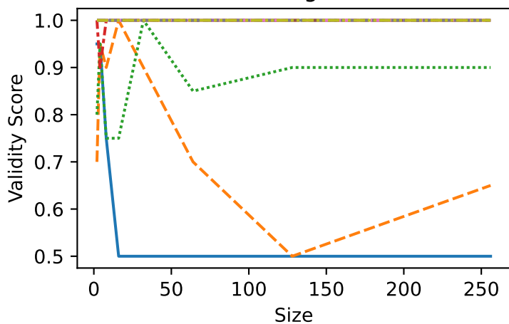
NumberWords
