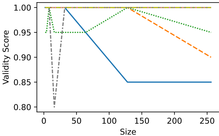
Int-n1000:1000
