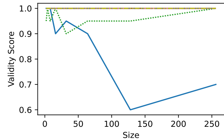
Float-10000000:10001000
