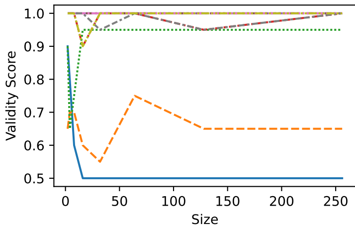
NumberWords
