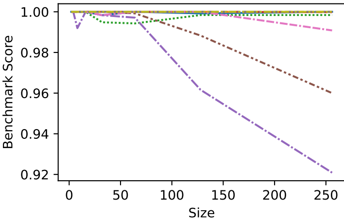
Float-10000000:10001000
