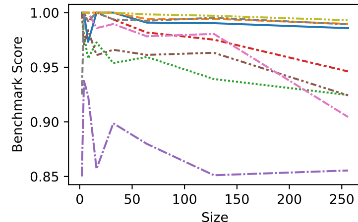
NumberWords
