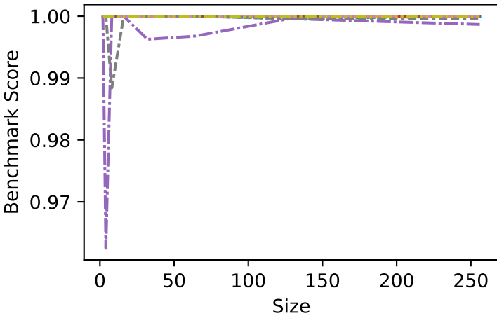
Int-n1000:1000
