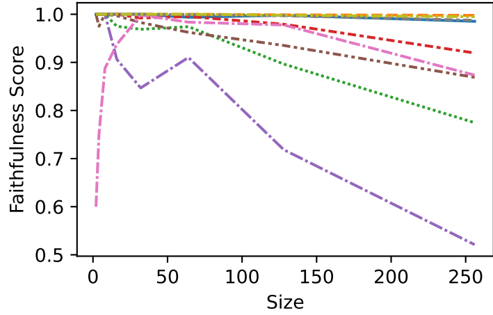
NumberWords
