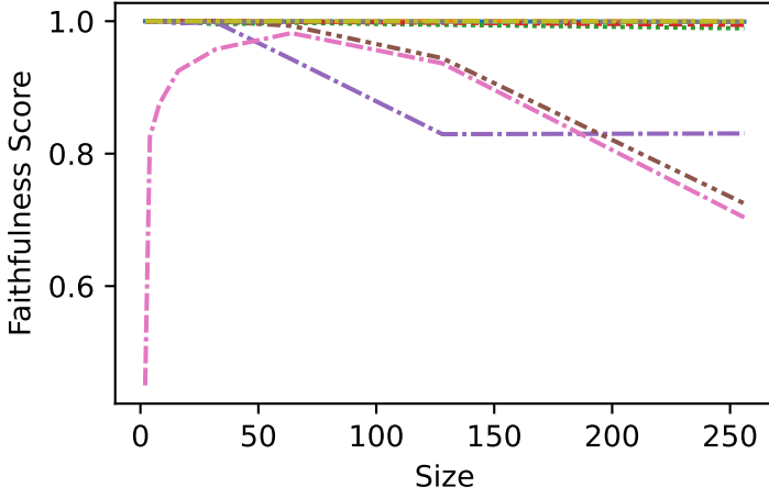
Float-10000000:10001000
