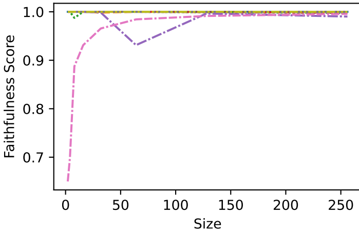
Int-n1000:1000
