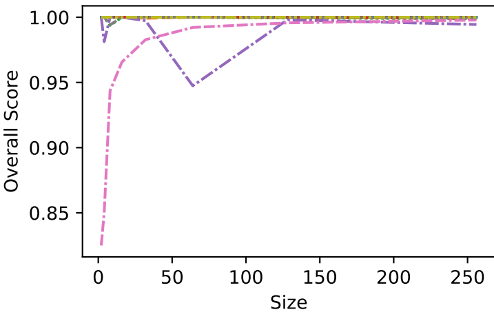
Int-10000000:10001000
