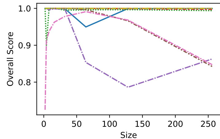
Int-n1000:1000
