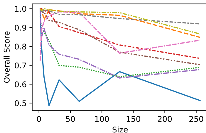
NumberWords
