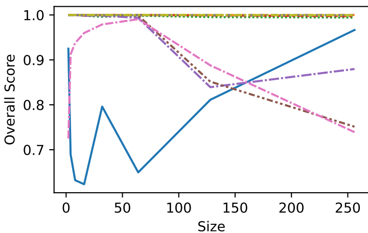
Float-10000000:10001000
