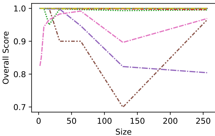
Int-n1000:1000
