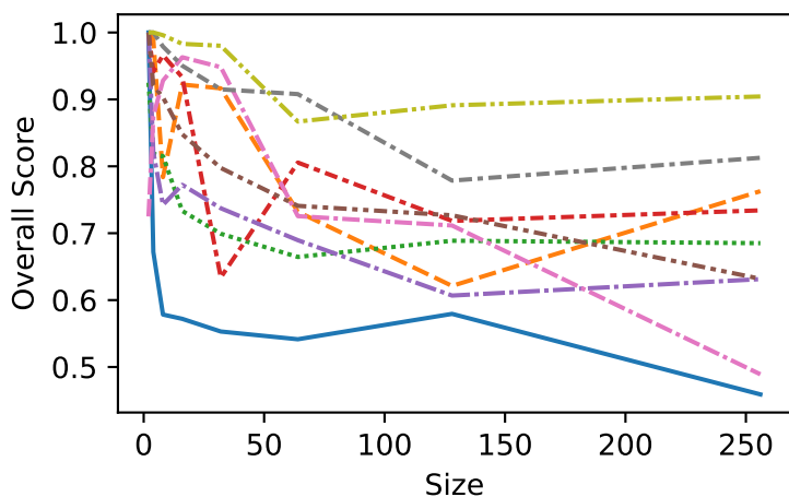
NumberWords
