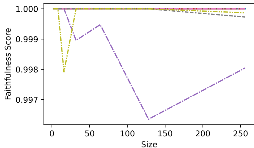
Faithfulness Score Filter Lower (basic)
