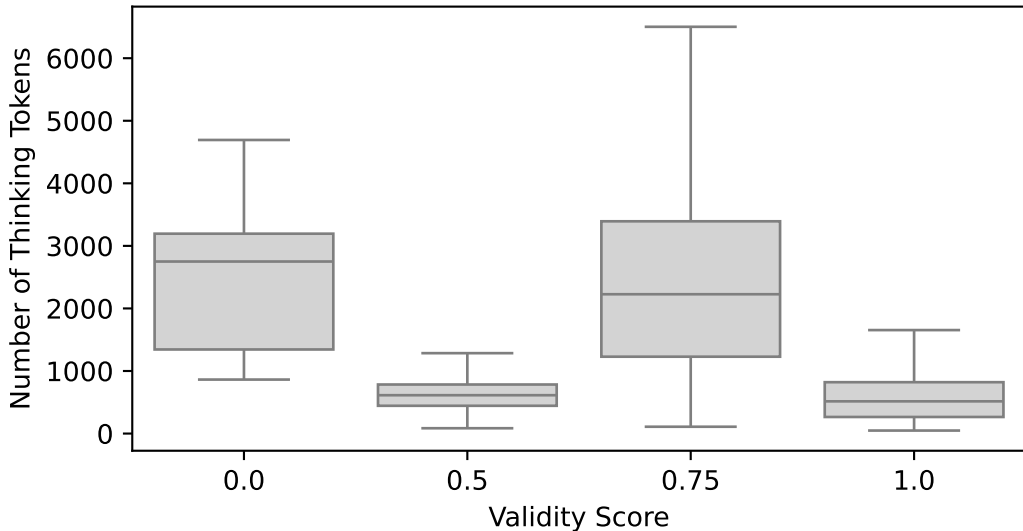
Thinking Length for Claude-4.5-Haiku-RE
