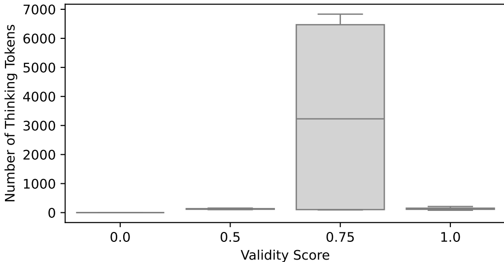
Thinking Length for Gemini-3-pro-RL
