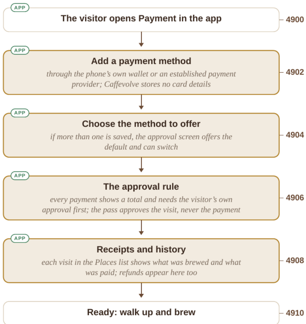
FIG. 46B. Setting up payment in the app.
