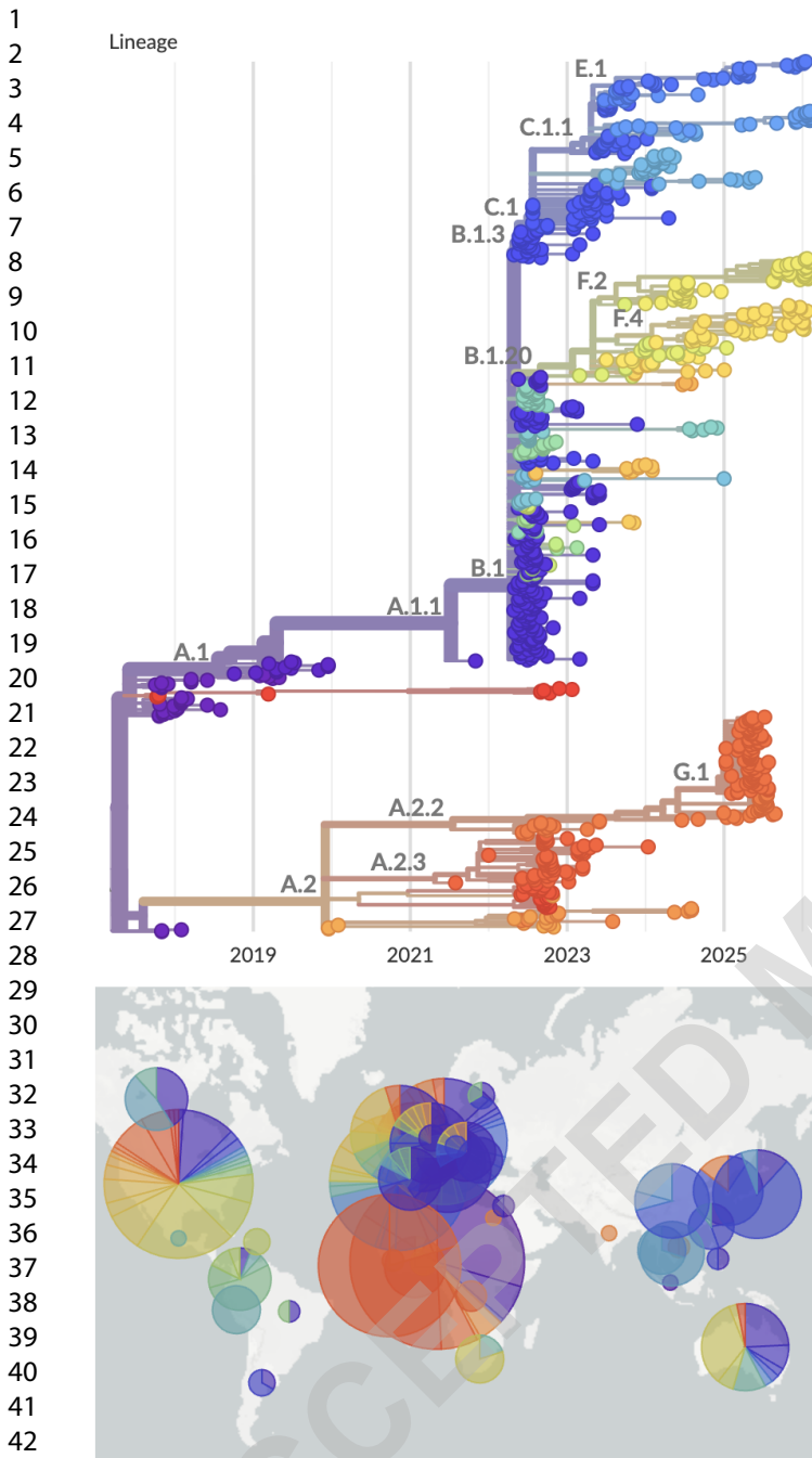
Figure 3 Time-resolved phylogeny of mpox clade IIb showing 927 viruses colored by lineage along with their geographic distribution. Branches shown have APOBEC3 mutation patterns distinct from ancestral branches (O'Toole et al., 2023), and so this is believed to represent human-to-human transmission starting in late 2017. A live version of this analysis is viewable at https://nextstrain.org/mpox/clade-IIb . Screenshot is from March 9, 2026.
