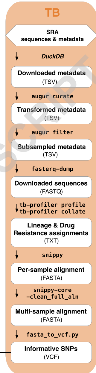
Figure 1 Outline of major steps for Nextstrain real-time analysis pipelines for viral and bacterial pathogens. Each pipeline is customized to the pathogen of interest, and the steps illustrated here represent those commonly shared across pipelines. The steps are arranged by the Snakemake workflows in which they occur within the pipelines, with each workflow shown as a colored block. The left hand arrow indicates that the outputs of the ingest workflow are used as inputs for the phylogenetic workflow of the viral pipeline. The right hand arrow indicates that the final steps of the bacterial pipeline are the same as those of the phylogenetic workflow of the viral pipeline; the arrow marks the point at which the two pipelines converge. The bacterial workflow is customized for Mycobacterium tuberculosis .
