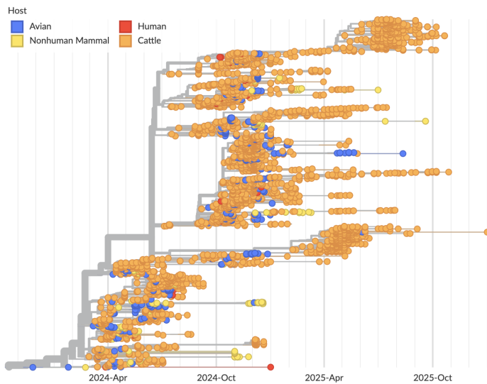
Figure 4 Full genome time-resolved phylogeny of avian influenza H5N1 outbreak in North America colored by host. A live version of this analysis is viewable at https://nextstrain.org/avian-flu/h5n1-cattle-outbreak/genome . Screenshot is from March 9, 2026.
