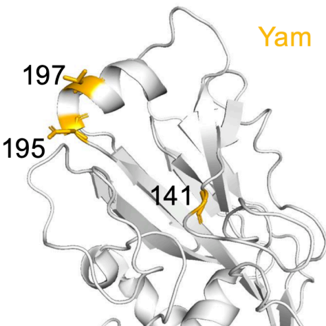
Supplemental Figure 1. Structurally homologous locations of egg-adaptive mutations in HA1. Residues that get egg-adaptive mutations in both influenza A viruses (top row) or both influenza B viruses (bottom row) are highlighted on the structure of HA. Egg-adaptive amino acids observed at these homologous sites in both viruses are listed in the table. Influenza A
