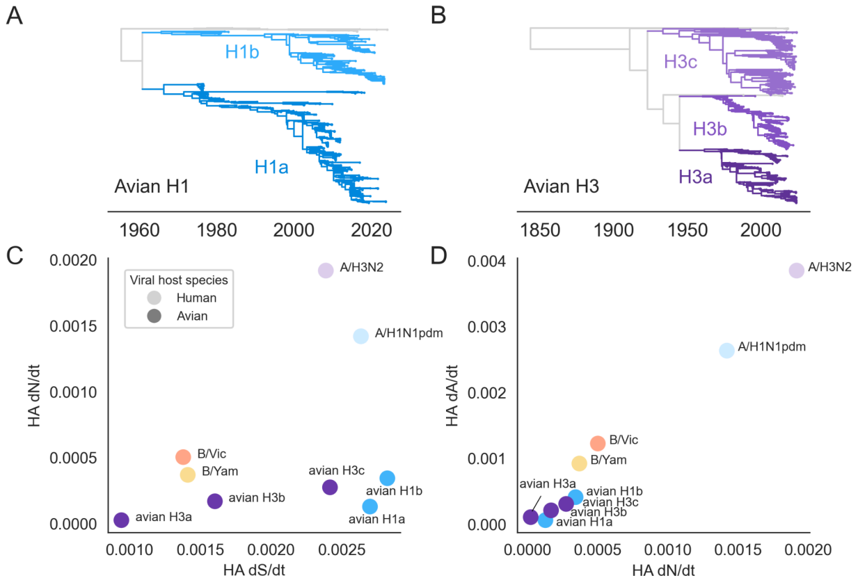
Supplemental Figure 10. Avian influenza A viruses have slower rates of nonsynonymous mutation and adaptive evolution than their human counterparts. A) Phylogeny of 899 avian H1 sequences, showing our designation of lineages H1a and H1b. B) Phylogeny of 1284 avian H3 sequences, showing our designation of lineages H3a, H3b, and H3c. C) Comparison of rates of synonymous and nonsynonymous mutation in hemagglutinin (HA) of four human influenza viruses (lighter shading) and five lineages of avian influenza A (darker shading). D) Comparison of the rate of nonsynonymous mutation and rate of adaptation evolution in HA of the same human and avian influenza viruses. Rates of synonymous and nonsynonymous mutation (per nucleotide per year) are calculated relative to the inferred ancestral sequence of that viral species, or lineage. Rates of adaptation across HA (in units of adaptive mutations per codon per year) are calculated according to the method in Kistler and Bedford 2023 37 .
