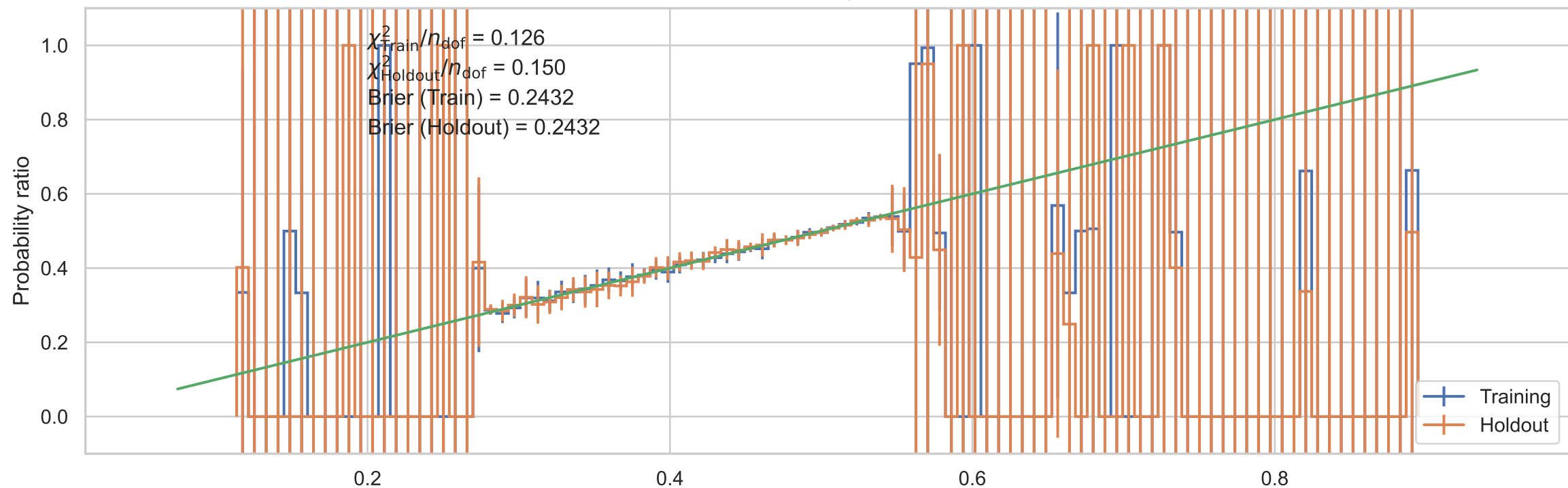
Calibration Curve , minus model
