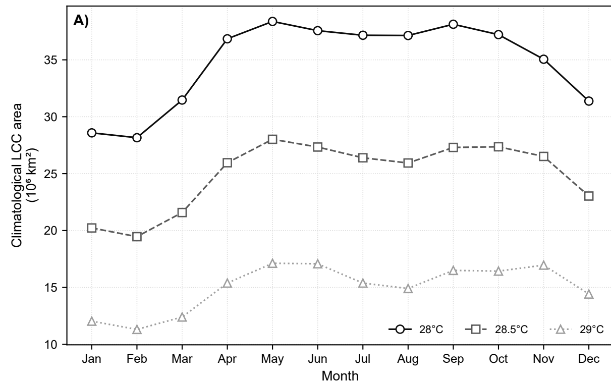
Seasonality and low-frequency evolution of PWP-LCC area
