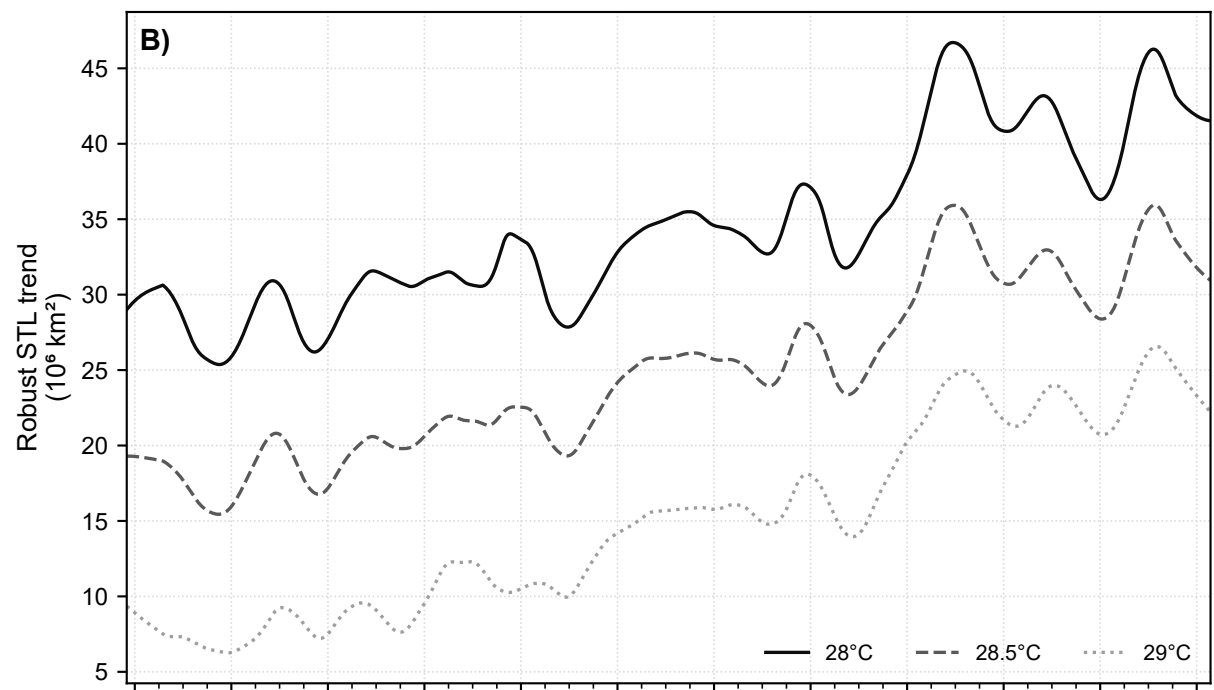
Seasonality and low-frequency evolution of PWP-LCC area
