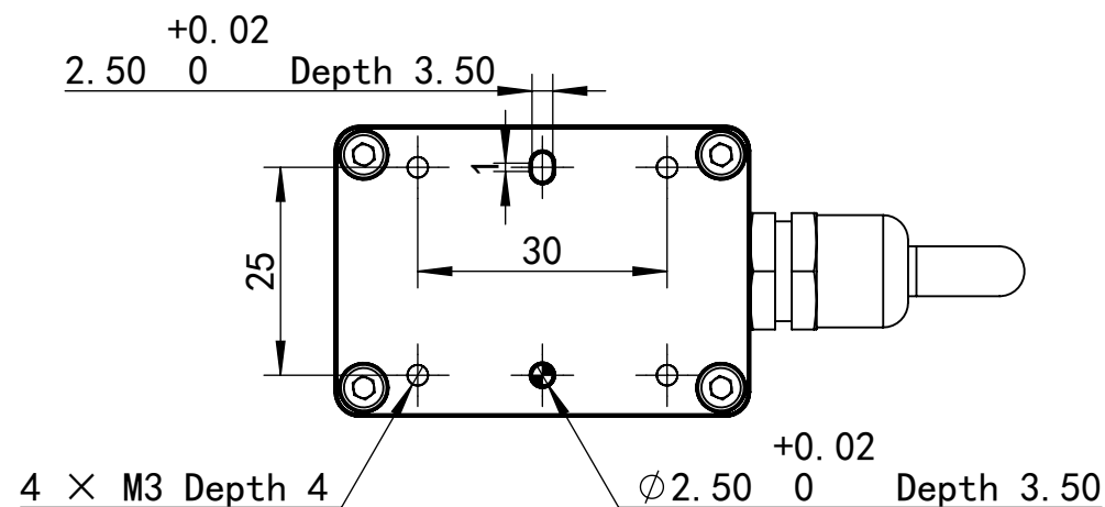
B-Direction View
