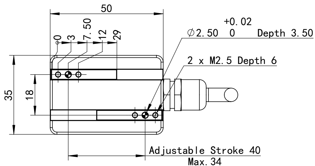
A-Direction View
