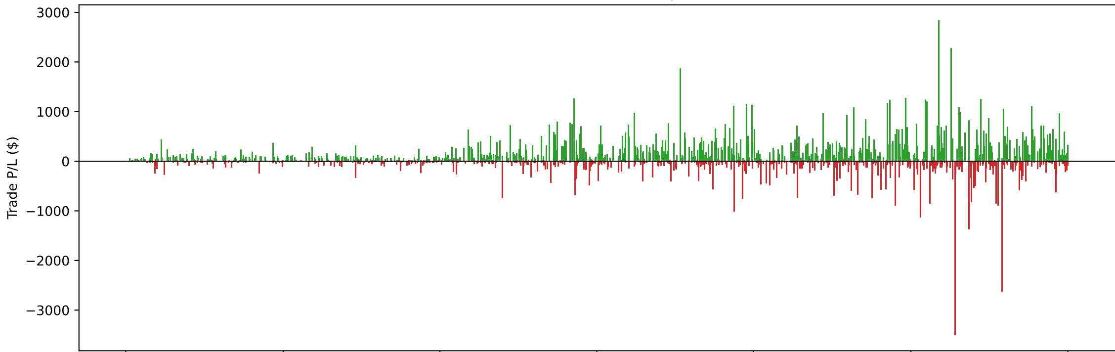
EURUSD Trade Profit/Loss per Exit
