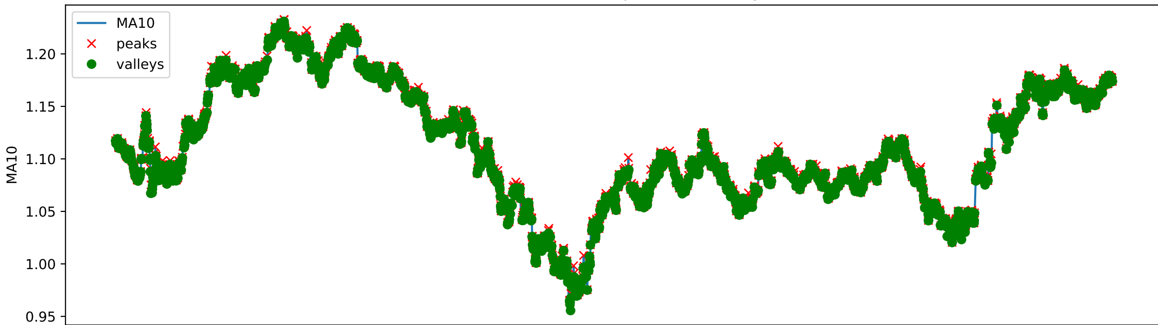
EURUSD MA10 with peaks and valleys
