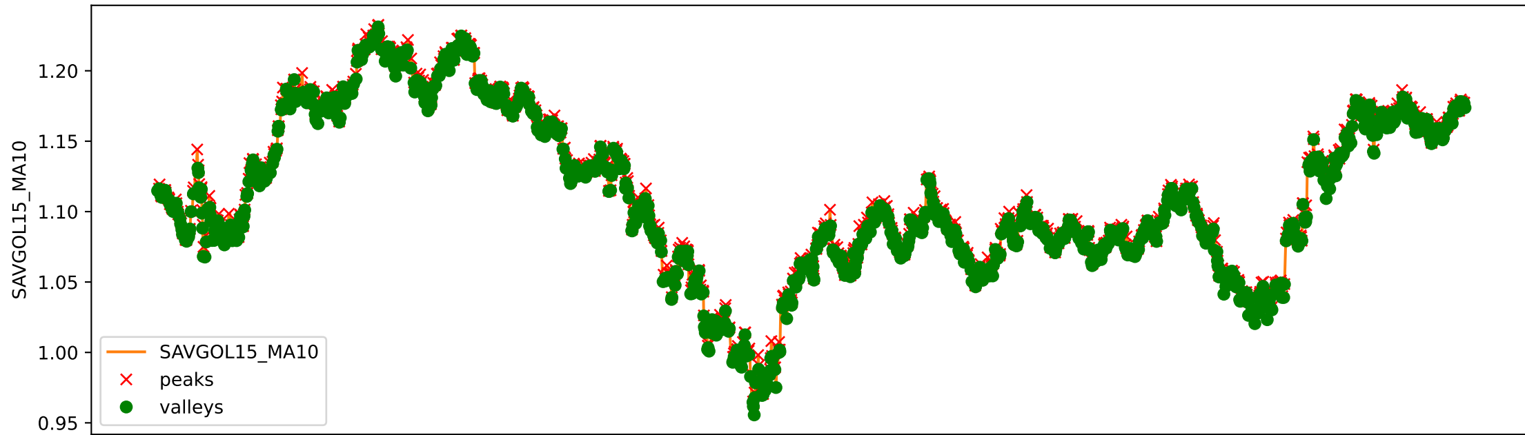
EURUSD Savitzky-Golay (input: MA10) with peaks and valleys
