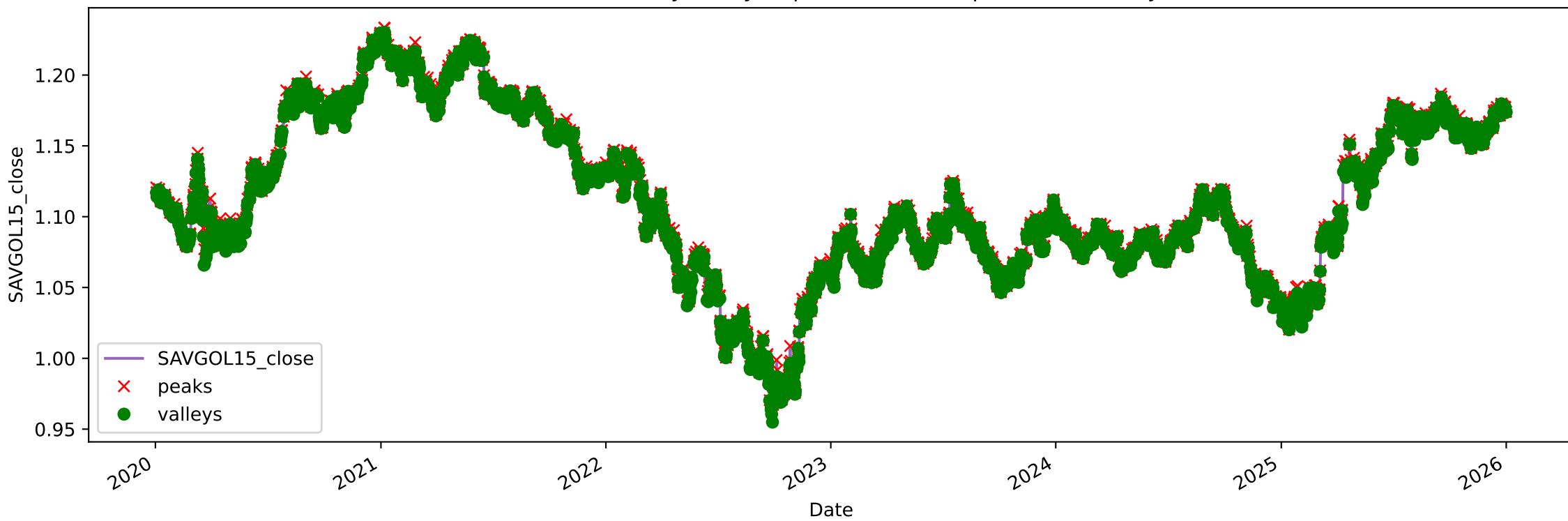
EURUSD Savitzky-Golay (input: close) with peaks and valleys
