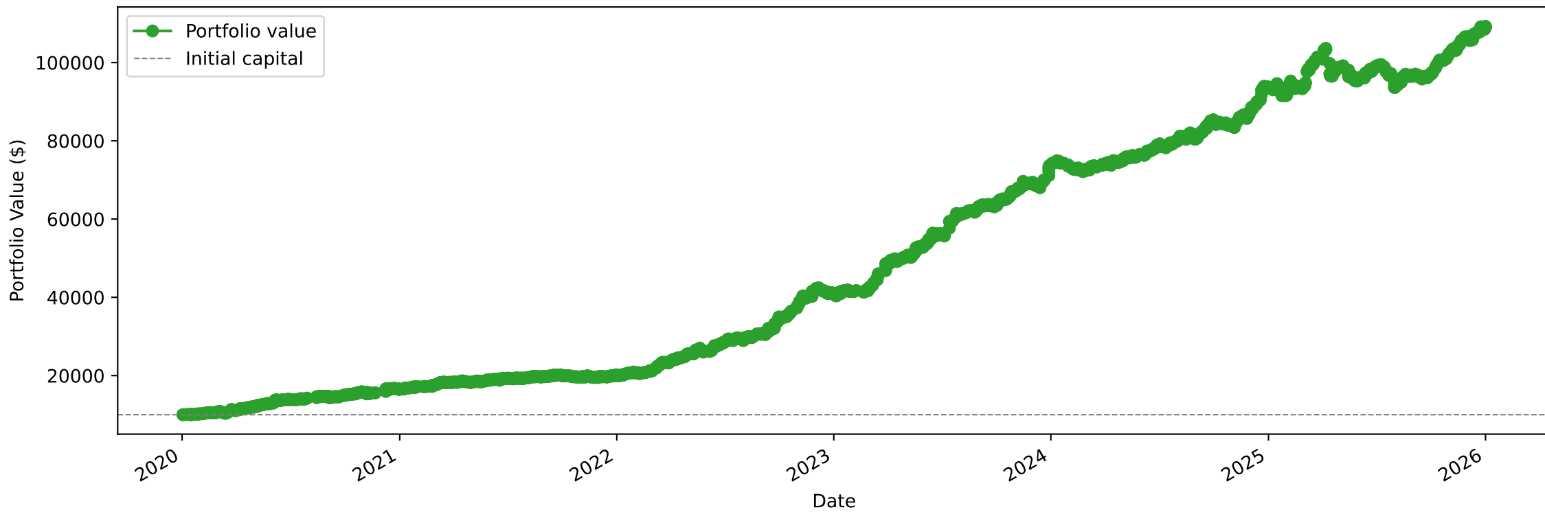
EURUSD Portfolio Value (start $10,000)
