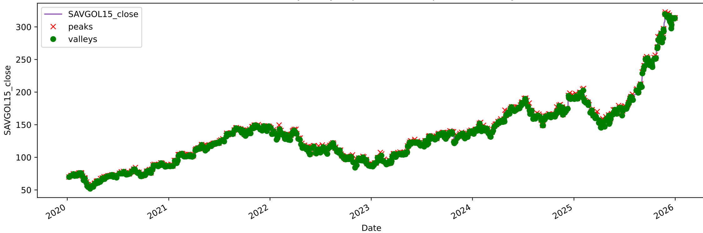
GOOGL Savitzky-Golay (input: close) with peaks and valleys
