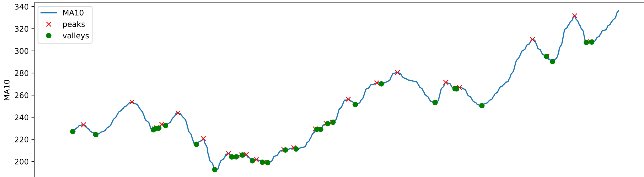
AAPL MA10 with peaks and valleys
