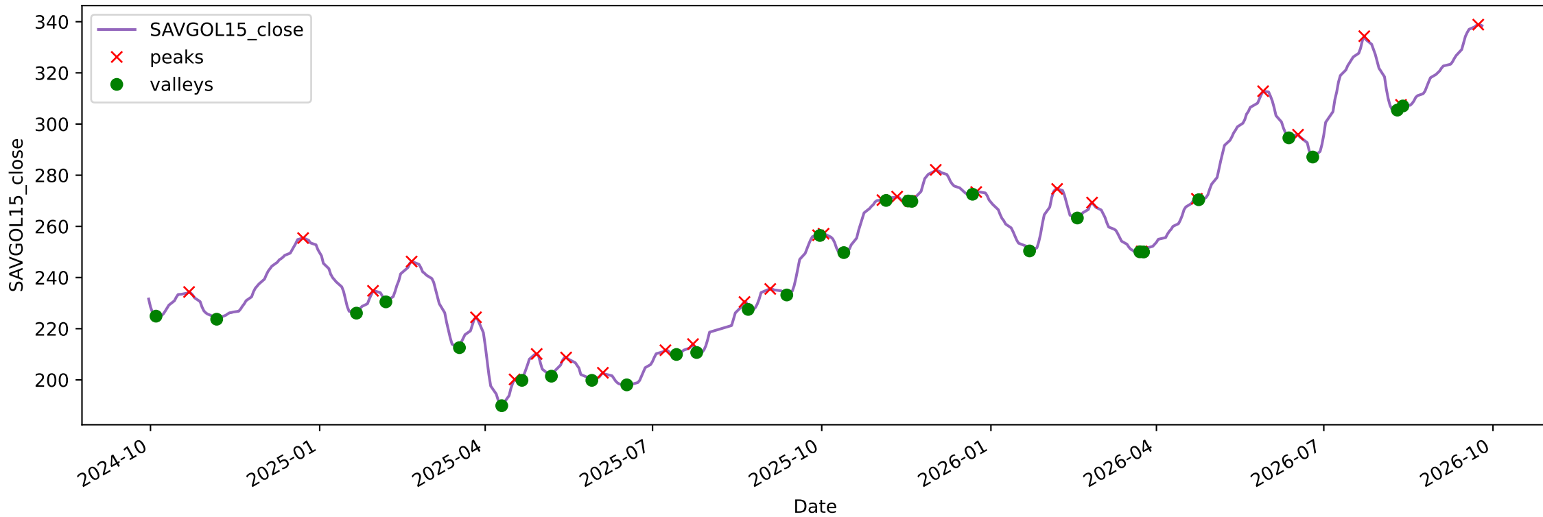
AAPL Savitzky-Golay (input: close) with peaks and valleys
