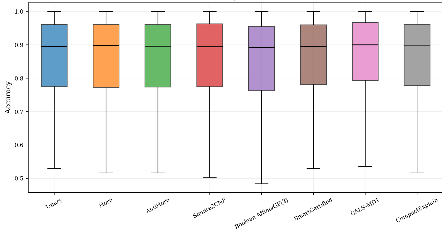
Accuracy boxplot
